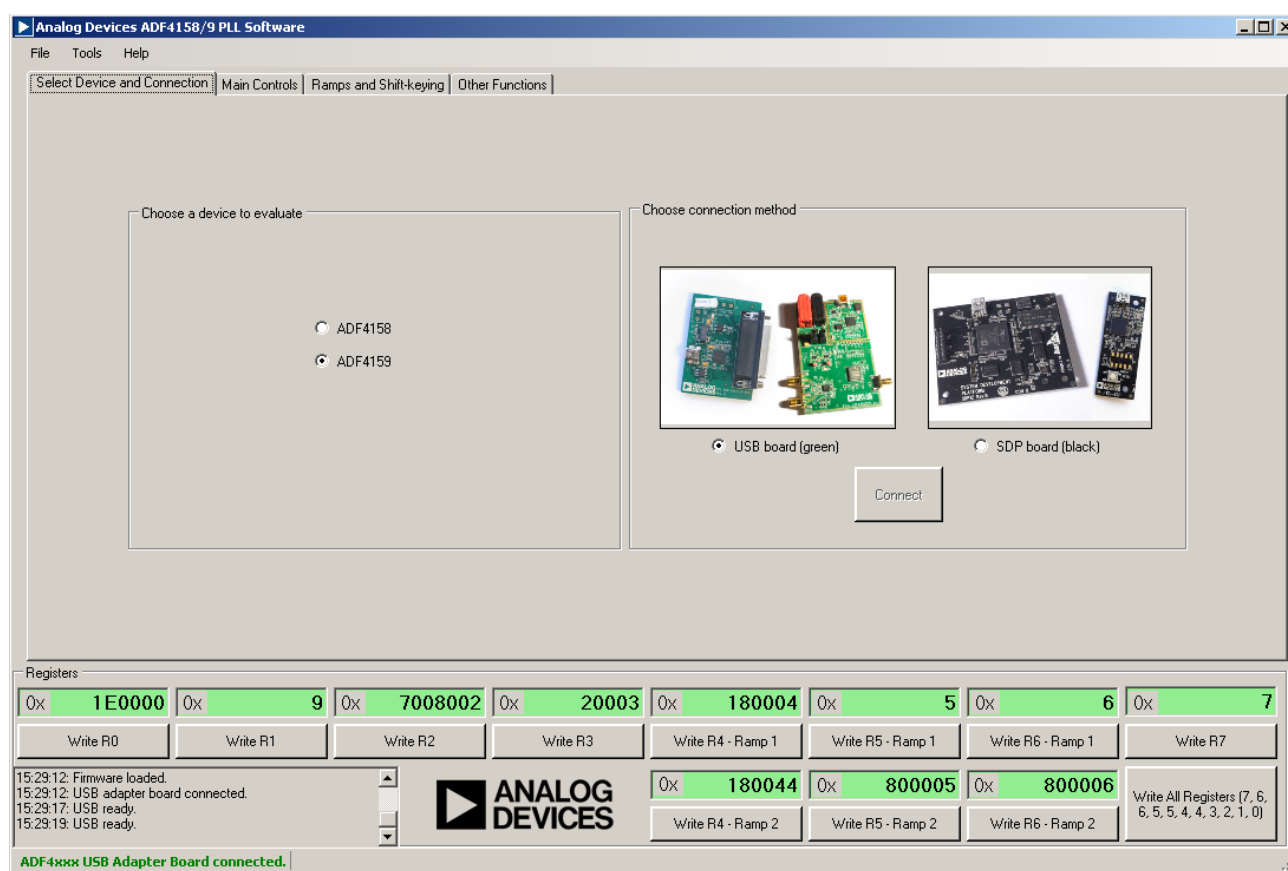
Figure 6. Software—Device Selection
