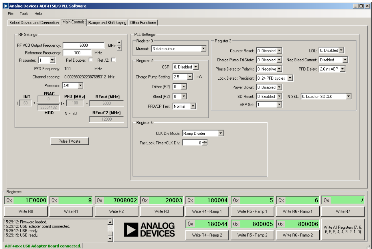
Figure 7. Software—Main Controls
